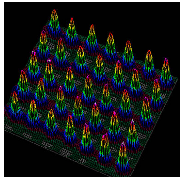
Figure 4. Experimental demonstration of spatial soliton arrays of partially incoherent light. Reproduced with permission from [116]. Copyright 2002 The Optical Society.
