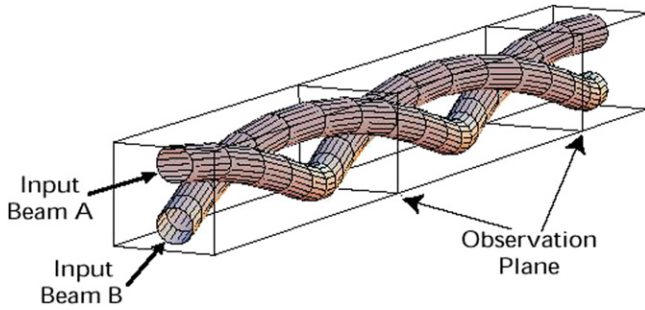
Figure 2. An illustration of spiraling collision of interacting spatial solitons as demonstrated in the experiment with photorefractive solitons [31]. The arrows at input indicate the initial launching directions of the two soliton beams. Reproduced with permission from [31]. Copyright 1997 American Physical Society.
