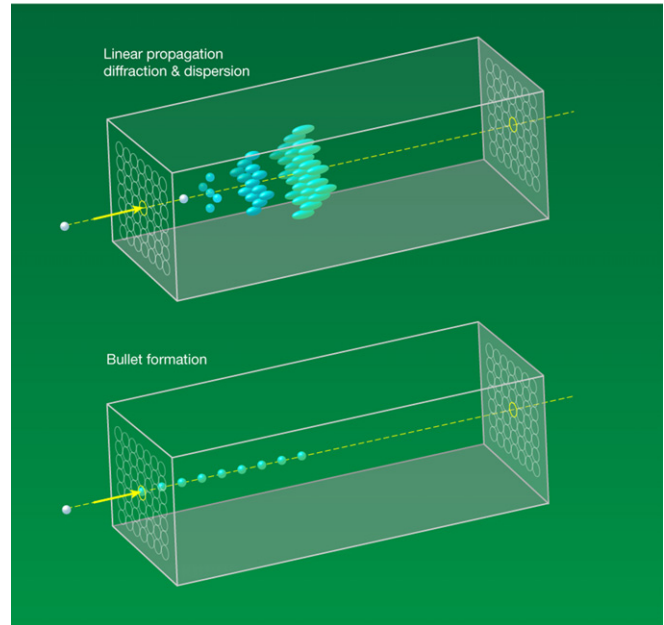
Figure 10. Illustration of 3D light bullets as observed in experiment with fs laser pulses propagating through a hexagonal array of glass waveguides. (top) A pulse undergoes spreading in both space and time during propagation in the waveguide array. (bottom) Nonlinear effects cause the light packet to remain stable and compact as it moves [267, 268]. Image courtesy of Alan Stonebraker. Reproduced with permission from [268]. Copyright 2010 American Physical Society.
