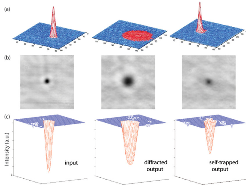
Figure 3. Experimental demonstration of self-trapping of (a) a 2D incoherent white-light beam and (b), (c) of a partially incoherent dark (vortex) beam. The top panels (a) show measured 3D intensity patterns of a white-light beam at input, linear output and nonlinear output positions, and the middle and bottom panels show 2D transverse patterns and 3D intensity plots of an incoherent vortex beam [99, 100]. Reproduced with permission from [100]. Copyright 1998 American Association for the Advancement of Science.
