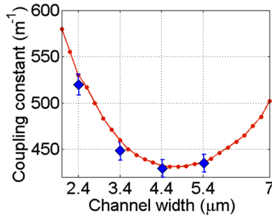
Fig. 11. The dependence of the coupling constant C on the ridge width with fixed center-to-center channel spacing of 10 \mu\text{m} . Data given by diamonds \blacklozenge , and calculations by the solid line.
